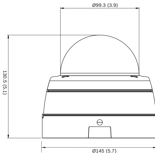
Dimensions (mm)
