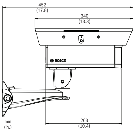
DINION capture 5000, vista laterale
