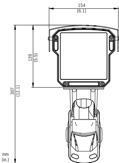
DINION capture 5000, vista anteriore
