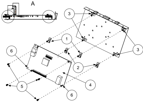
Figure 2: Optional Mounting Plate
