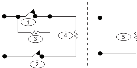
Figure 12.1: Dual EOL resistor option
