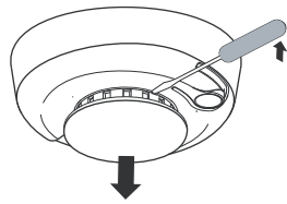
Figure 8.2: Remove the detector cap
