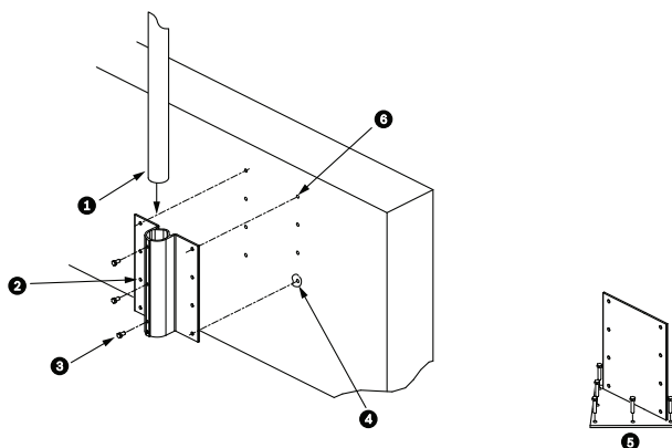
Figure 8.1: Support de montage parapet et platine de montage parapet
